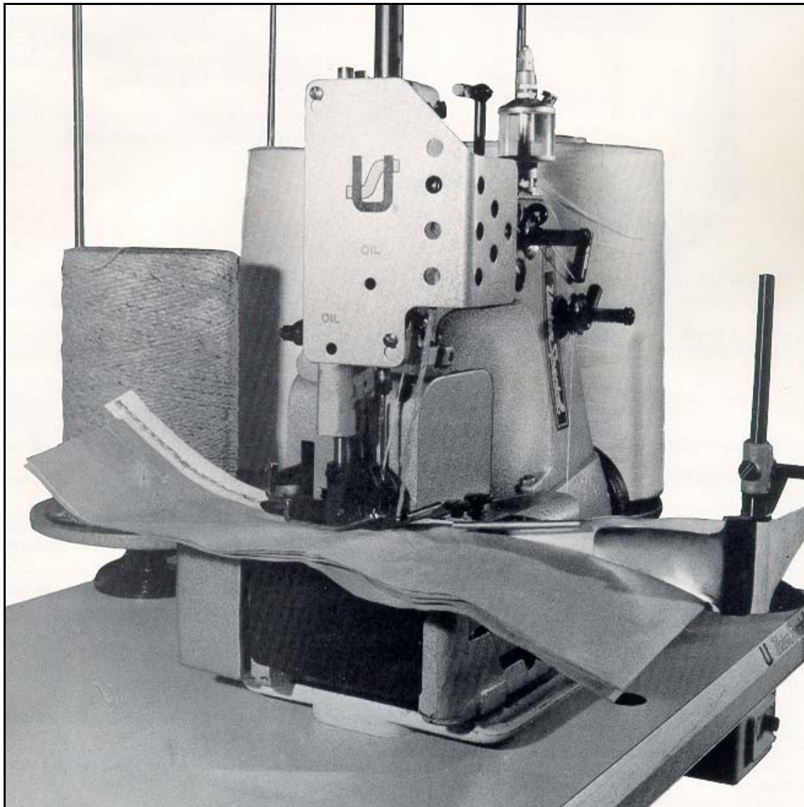
80800HAZ3381 with Sewing Table UN382G130
